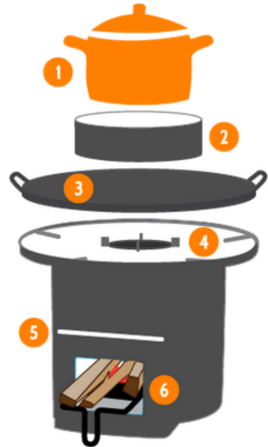
Rocket Stove
